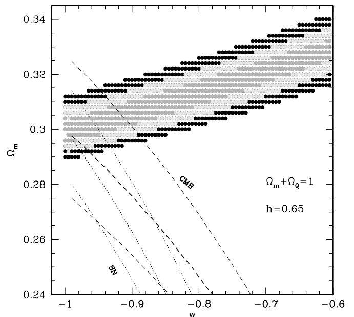
FIG. 16.—Likelihood contours for a fixed h = 0.65 as in Fig. 9, but zooming in for clarity. Also shown are combinations of w and \Omega_m that keep the spherical harmonic index l of the first Doppler peak in the CMB anisotropy data constant to within \pm 1\% (dashed lines) and combinations that keep the luminosity distance to redshift z = 1 constant to the same accuracy.
