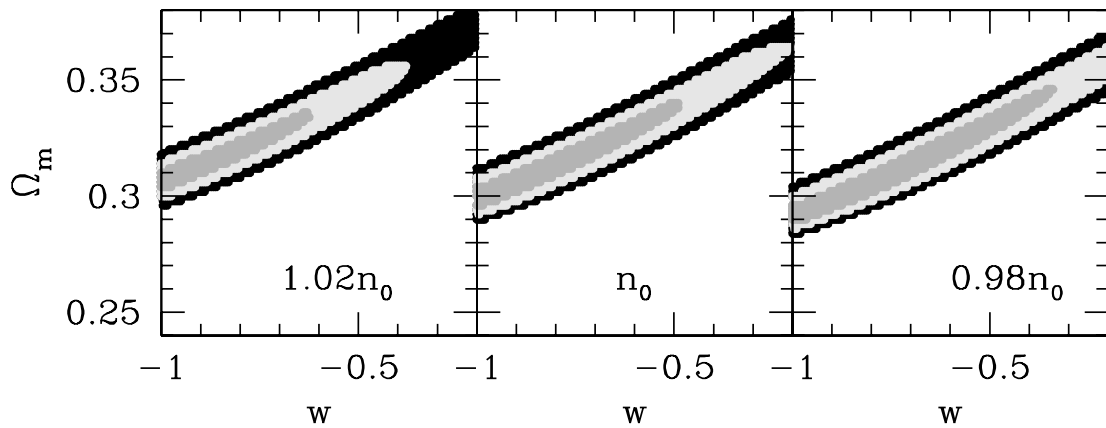
FIG. 14.—Middle panel shows the likelihood contours for a fixed h = 0.65 in the X-ray survey, as in Fig. 9. The left- and right-hand panels show the deviations in the contours caused by a \pm 2\% offset in the local cluster abundance determination.
