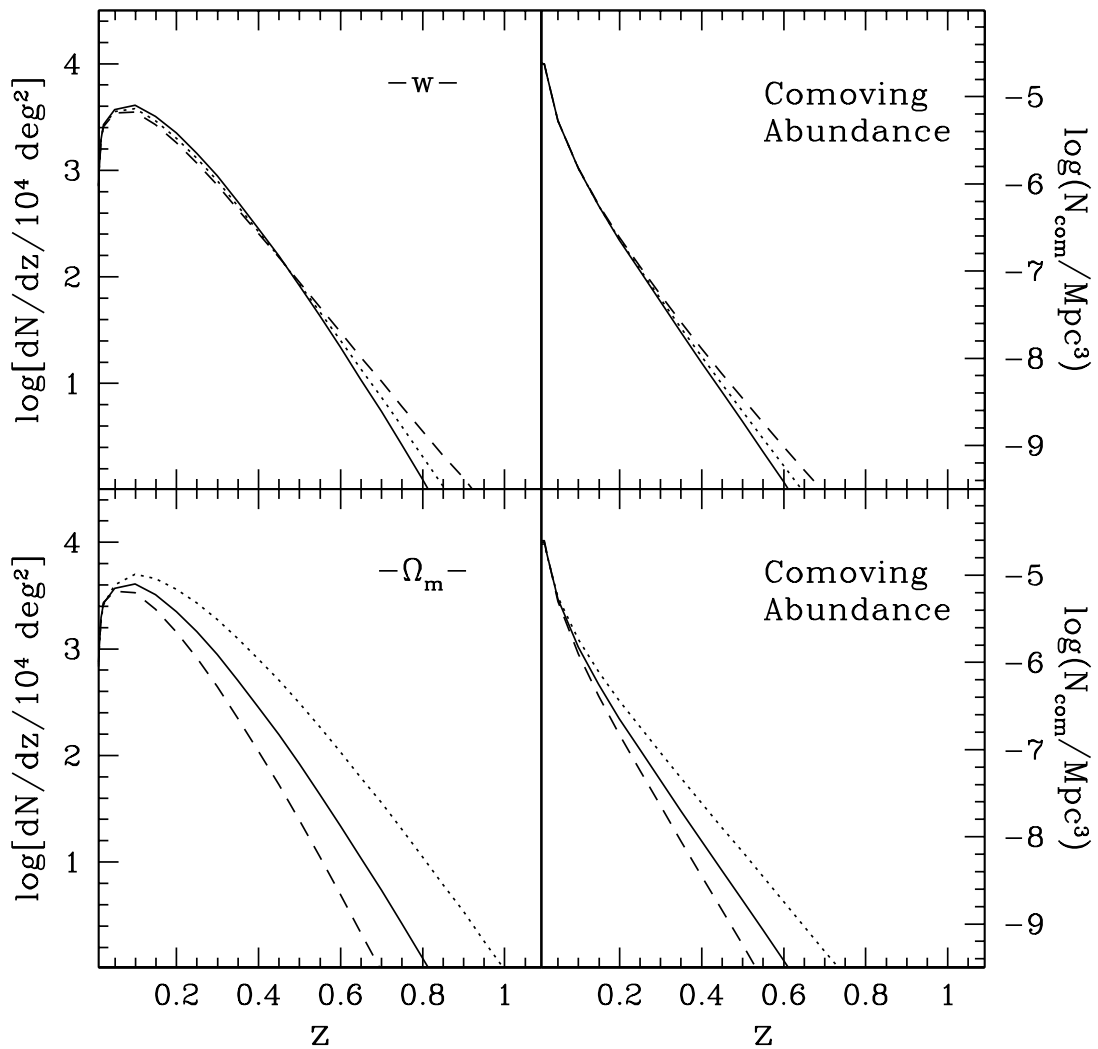
FIG. 7.—Effect of changing w (upper panels) or \Omega_m (lower panels) when all other parameters are held fixed in an X-ray survey, and the survey mass limit is held fixed at its fiducial value, irrespective of cosmology. A comparison with Fig. 6 shows that nearly all of the w -sensitivity is accounted for by the cosmology-dependence of the limiting mass. On the other hand, the \Omega_m -sensitivity is caused mostly by the growth function.
