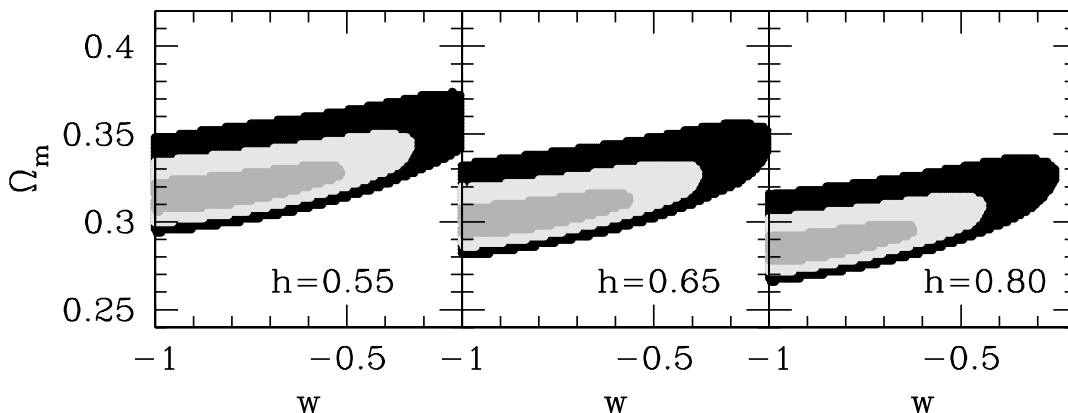
FIG. 8.—Contours of 1, 2, and 3\sigma likelihood for different models when they are compared to a fiducial flat \Lambda CDM model with \Omega_m = 0.3 and h = 0.65 , using the SZE survey. The three panels show three different cross sections of constant total probability at fixed values of h (0.55, 0.65, and 0.80) in the investigated three-dimensional \Omega_m, w, h parameter space.
