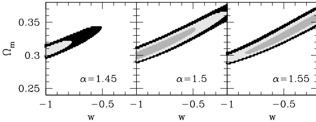
FIG. 13.—Middle panels show the likelihood contours for a fixed h = 0.65 in the X-ray survey, as in Fig. 9. The other two panels show the deviations caused by an offset in the slope M \propto T^\alpha .
