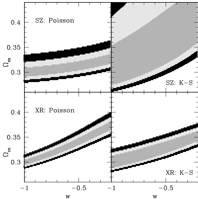
FIG. 10.—Likelihood contours of 1, 2, and 3 \sigma probabilities as in Figs. 8 and 9, but when only the total number of clusters ( left-hand panels ) or only the redshift distributions ( right-hand panels ) are used to compute the likelihoods between two models.
