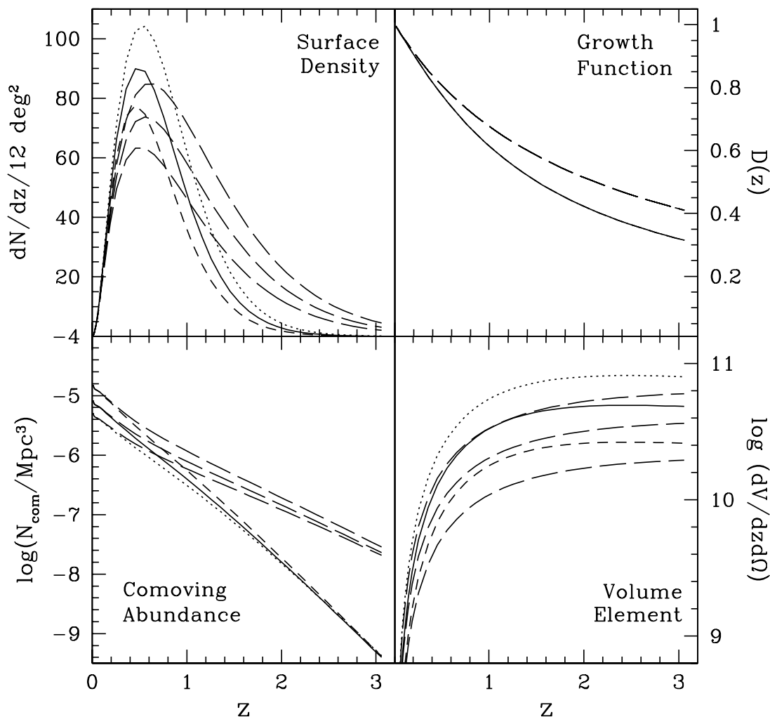
FIG. 4.—Effect of changing h when all other parameters are held fixed. The \Lambda CDM model of Fig. 3 is shown (solid curve) together with models with h = 0.55 (dotted curve); h = 0.80 (short-dashed curve); and OCDM models with h = 0.55, 0.65, 0.80 (long-dashed curves, top to bottom).
