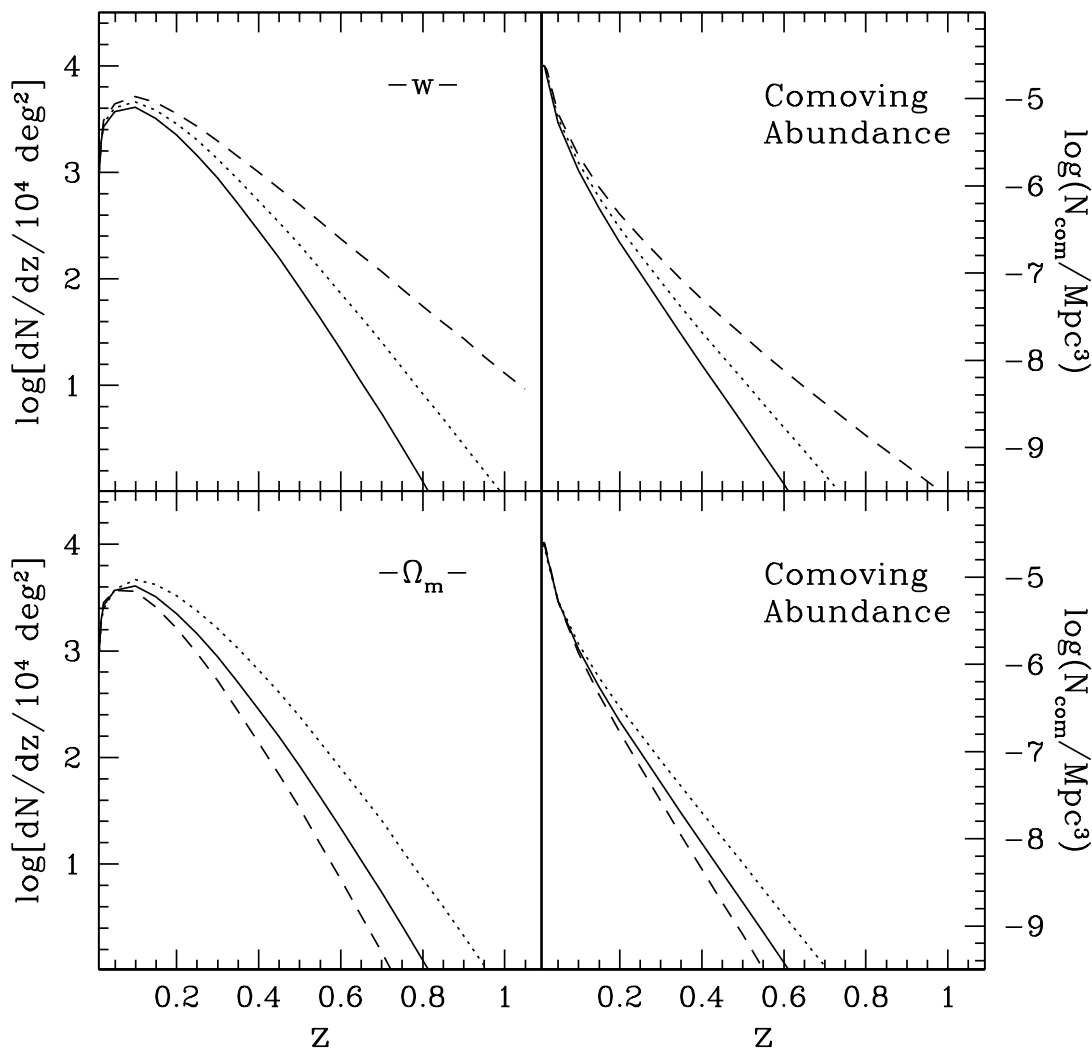
FIG. 6.—Effect of changing w (upper panels) or \Omega_m (lower panels) when all other parameters are held fixed in the X-ray survey. Note the much larger numbers of clusters in comparison to the SZE survey. In the top panel, the curves correspond to w = -1 (solid curve), w = -0.6 (dotted curve) and w = -0.2 (dashed curve). In the bottom panel, the curves correspond to \Omega_m = 0.3 (solid curve), \Omega_m = 0.27 (dotted curve) and \Omega_m = 0.33 (dashed curve).
