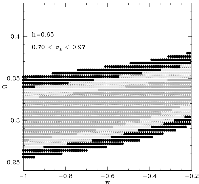
FIG. 15.—Likelihood contours for a fixed h = 0.65 in the X-ray survey, as in Fig. 9; however, we here considered \sigma_8 as a free parameter rather than fixing its value based on the local abundance. Models with \sigma_8 outside the range 0.7 < \sigma_8 < 0.97 resulted in likelihoods worse than 3\sigma .
