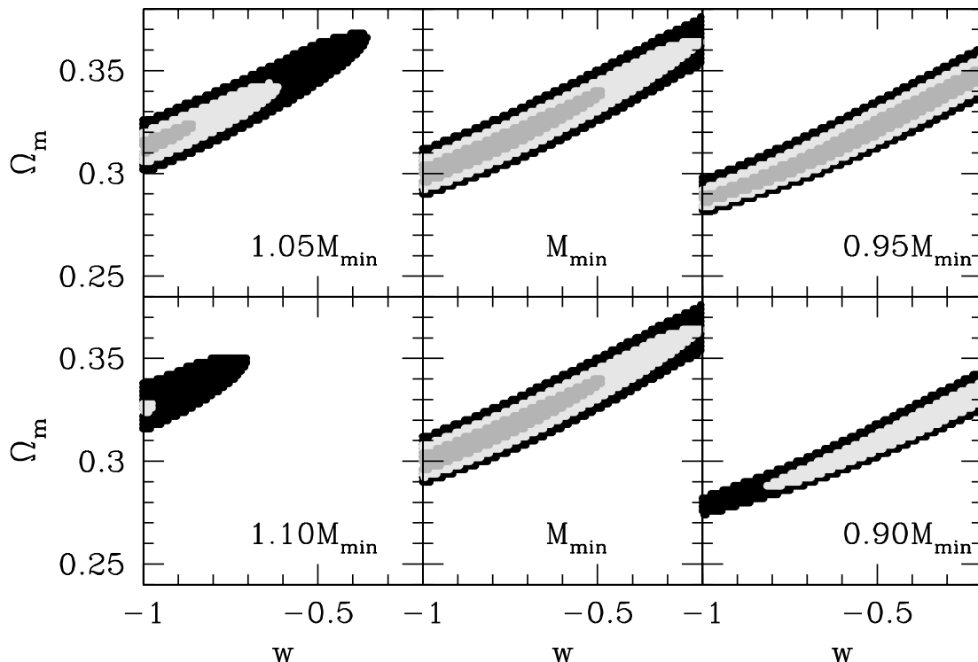
FIG. 12.—Middle panels show the likelihood contours for a fixed h = 0.65 in the X-ray survey, as in Fig. 9. The upper and lower panels show the deviations in the contours caused by either a \pm 5\% or a \pm 10\% offset in the M - T normalization.
