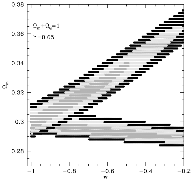
FIG. 11.—Likelihood contours for a fixed h = 0.65 in the X-ray survey, as in the middle panel of Fig. 9, but zooming in for clarity. The added (nearly horizontal) contours shows the allowed region when variations of the limiting mass with cosmology are not taken into account.
