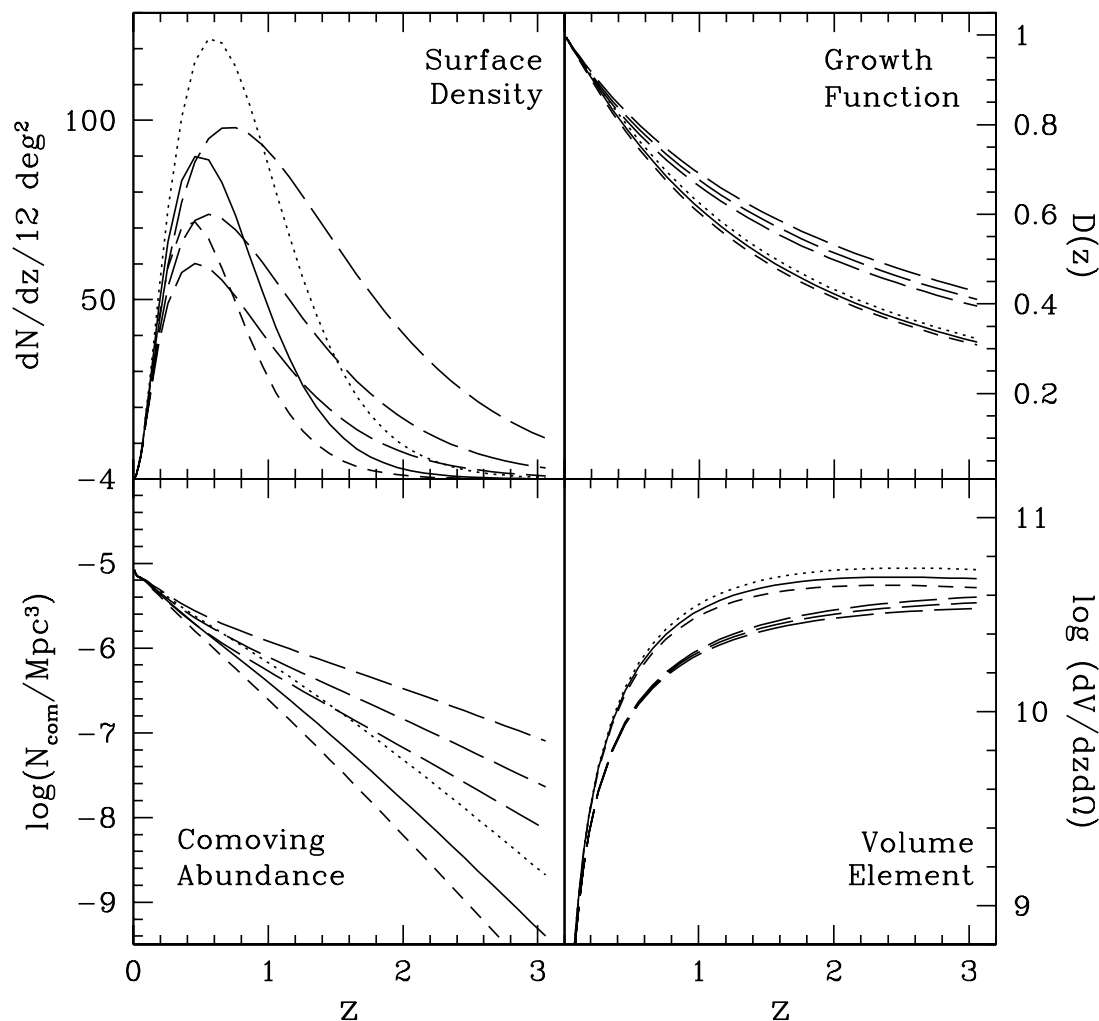
FIG. 2.—Effect of changing \Omega_m when all other parameters are held fixed. The four panels show (clockwise from upper left) the surface density of clusters at redshift z , the linear growth function, the volume element in units of \text{Mpc}^3 \text{sr}^{-1} \text{redshift}^{-1} , and the comoving cluster abundance. The solid curve shows our fiducial flat \Lambda CDM model, with w = -1 , \Omega_m = 0.3 , and h = 0.65 . Also shown are models with \Omega = 0.27 (dotted curve); \Omega = 0.33 (short-dashed curve); and OCDM models with \Omega = 0.27, 0.30, 0.33 (long-dashed curves, top to bottom).
