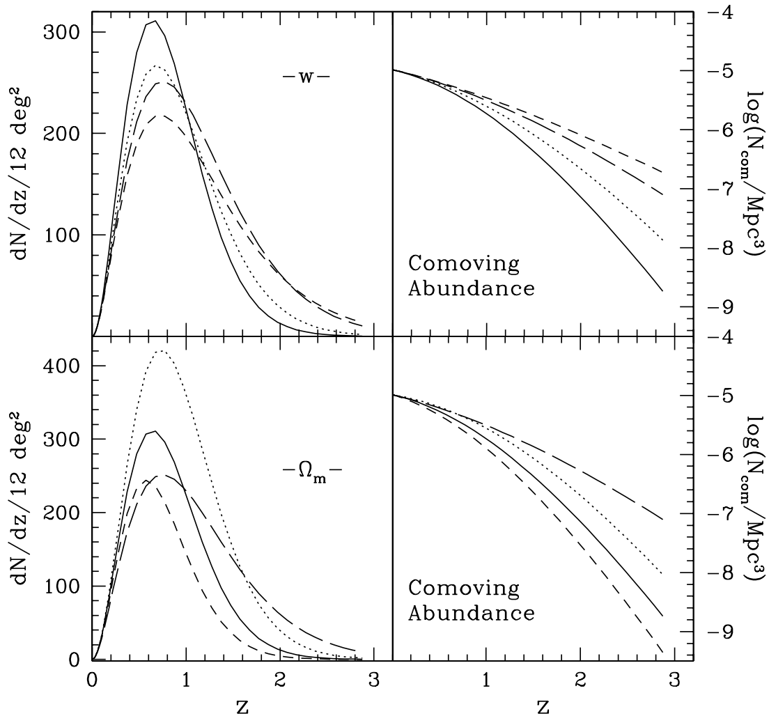
FIG. 5.—Effect of changing w (upper panels) or \Omega_m (lower panels) when all other parameters are held fixed, including the mass limit. The types of the curves correspond to the different models in the SZE survey, as shown in Figs. 2 and 3.
