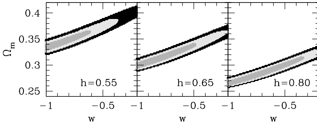
FIG. 9.—Contours of 1, 2, and 3 \sigma likelihood for models when they are compared to a fiducial flat \Lambda CDM model, as in Fig. 8, but for the X-ray survey
