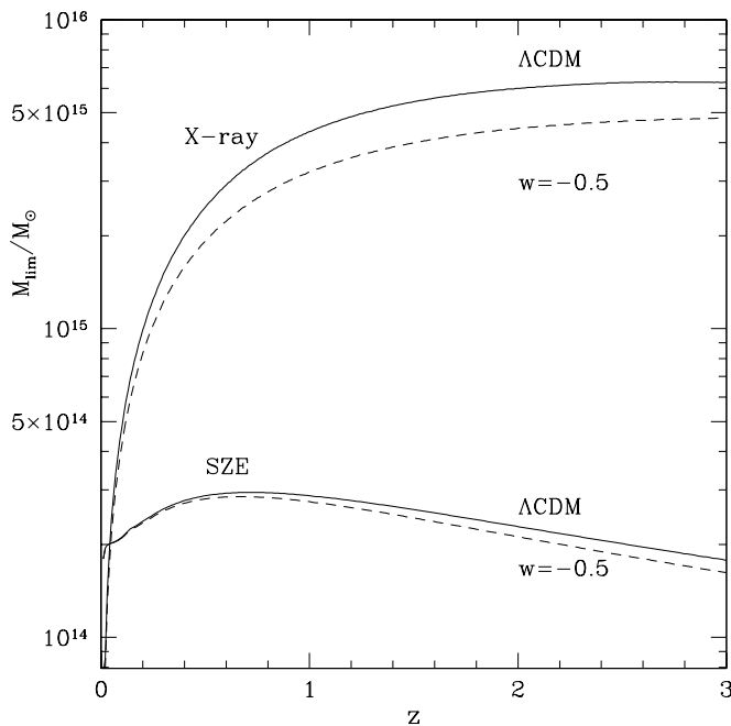
FIG. 1.—Limiting cluster virial masses ( M_{180} ) for detection in the X-ray survey (upper pair of curves) and in the SZE survey (lower pair of curves). The solid curves show the mass limit in our fiducial flat \Lambda CDM model, with w = -1 , \Omega_m = 0.3 , and h = 0.65 , and the dotted curves show the masses in the same model except with w = -0.5 .
