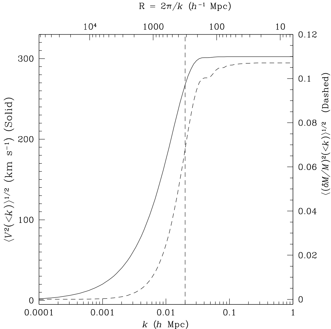
Fig. 1. The solid curve shows the square root of the contribution to the mean squared bulk flow within a tophat of radius 50 h^{-1} Mpc as a function of the lower cutoff in k , for a standard CDM model. The dashed line is the square root of the contribution to the mean squared mass fluctuations (right-hand scale). Note that the velocity field includes much more contribution from small k (large scales).
