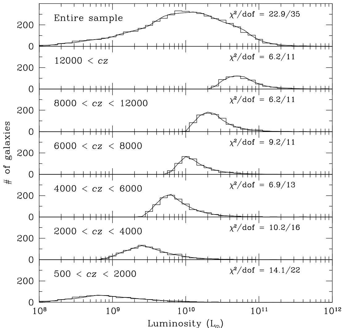
Fig. 4. The luminosity distribution (histogram) of the IRAS 1.2 Jy sample in different redshift ranges, together with the predicted distributions, given the luminosity function. The values of \chi^2/dof given in each panel refer to the difference between the two curves, with errors given by Poisson statistics.
