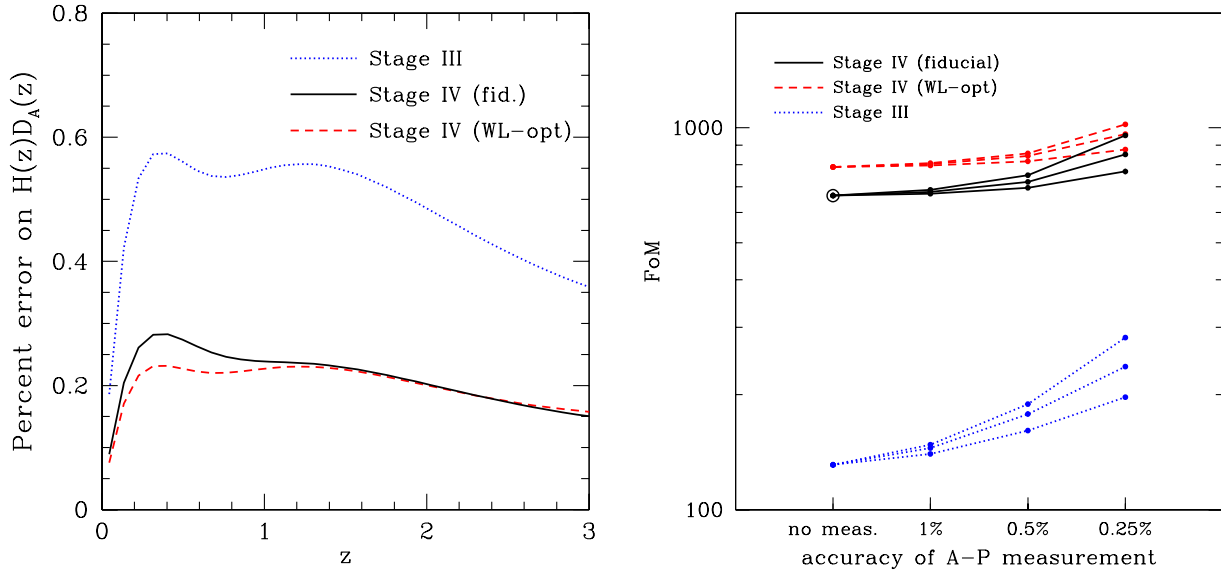
Figure 49 Left : Predicted fractional error ( 1\sigma ) of the AP parameter H(z)D_A(z) from our fiducial Stage III and Stage IV CMB+SN+BAO+WL programs, assuming a w_0-w_a dark energy parameterization. Right : Dependence of the DETF FoM on additional measurements of H(z)D_A(z) at a single redshift. For each forecast, the three curves from top to bottom assume AP measurements at z = 0.5 , z = 1 , and z = 2 , respectively.
