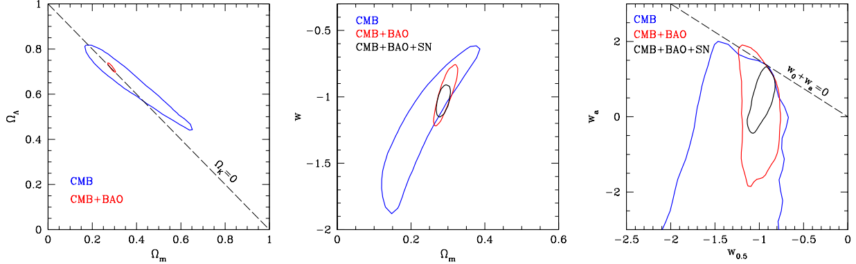
Figure 9 Constraints from combinations of current BAO data (the four points in the left hand panel of Fig. 8), WMAP7 CMB data, and Union2 SN data in (a) the (\Omega_m, \Omega_\Lambda) plane assuming w = -1 , (b) the (\Omega_m, w) plane assuming \Omega_k = 0 , and (c) the (w_{0.5}, w_a) plane assuming \Omega_k = 0 , where w_{0.5} is the value of w at z = 0.5 . Contours show 68% confidence intervals. We omit the CMB+BAO+SN combination from panel (a) because it is nearly identical to the CMB+BAO combination.
