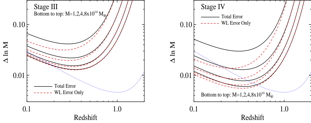
Figure 28 Mass uncertainty from stacked weak lensing calibration as a function of redshift, assuming only WL shape noise (dashed red curves) and including sample variance due to intrinsic scatter between WL mass and halo mass (solid curves). For Stage III data (left) we assume \sigma_e = 0.4 and \bar{n}_g = 10 galaxies/arcmin 2 , while for Stage IV (right) we assume \sigma_e = 0.3 and \bar{n}_g = 30 galaxies/arcmin 2 . For both cases we assume a 10^4 deg 2 survey, and the redshift bin width is z = z_c \pm 0.05 . Each curve corresponds to a different mass threshold as labeled. The blue dotted line shows the mass error corresponding to a statistics-limited cluster survey with a threshold mass of 10^{14} M_\odot , as per Figure 23. The intersection between the blue dotted line and the lowest solid black line marks the redshift at which a cluster abundance experiment with a threshold mass of 10^{14} M_\odot transitions from being dominated by the statistical error in cluster abundance (at low redshift) to the error in the weak lensing mass calibration (at high redshift).
